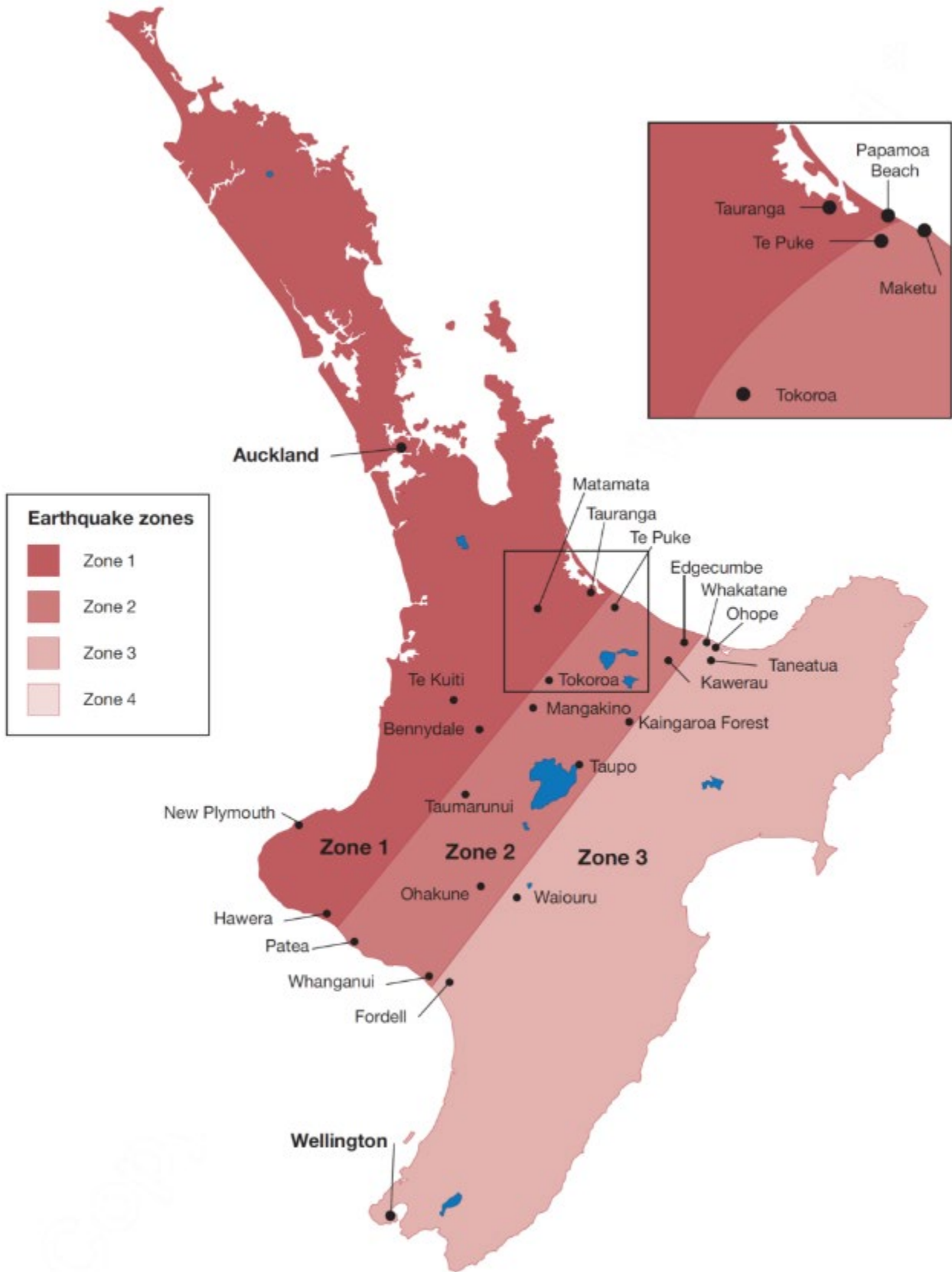
Figure 4.1 – Earthquake zones (North Island) (see 4.2.2)
