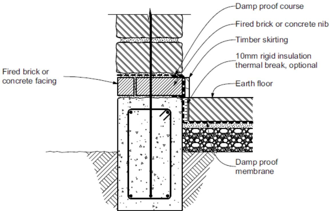
Figure 5.10 – Footing – Earth floor
