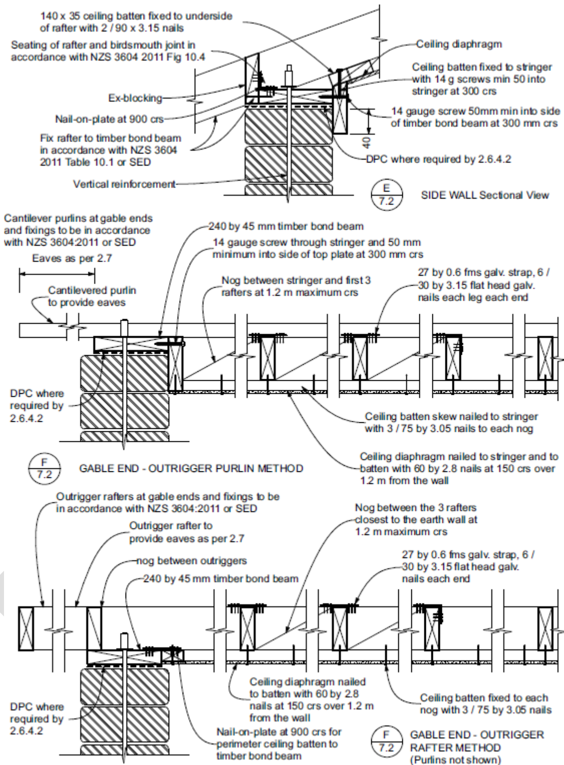
Figure 7.4 – Connection of ceiling diaphragms to side and gable end walls for sloping diaphragms on underside of rafters
