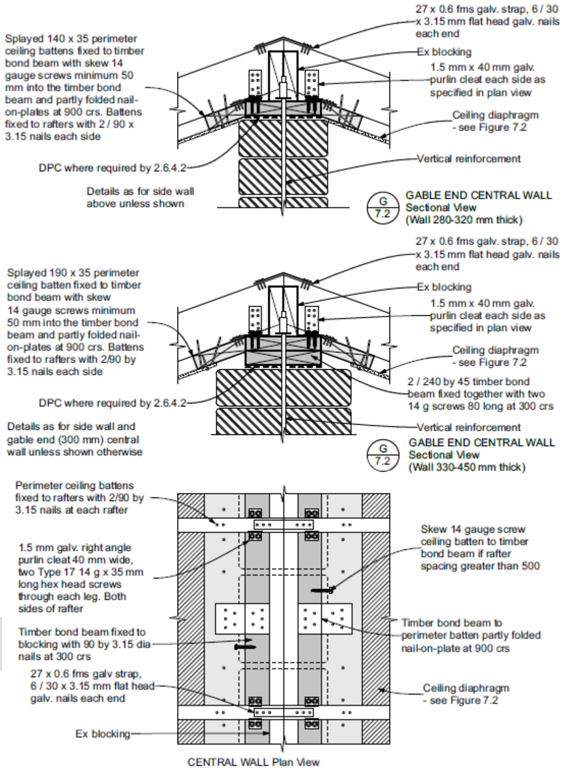
Figure 7.5 – Connection of ceiling diaphragms to central walls for sloping diaphragms on underside of rafters
