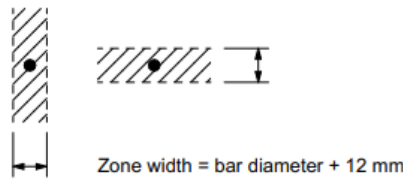
Figure 5.3 – Footing reinforcement in earthquake zone 1.
