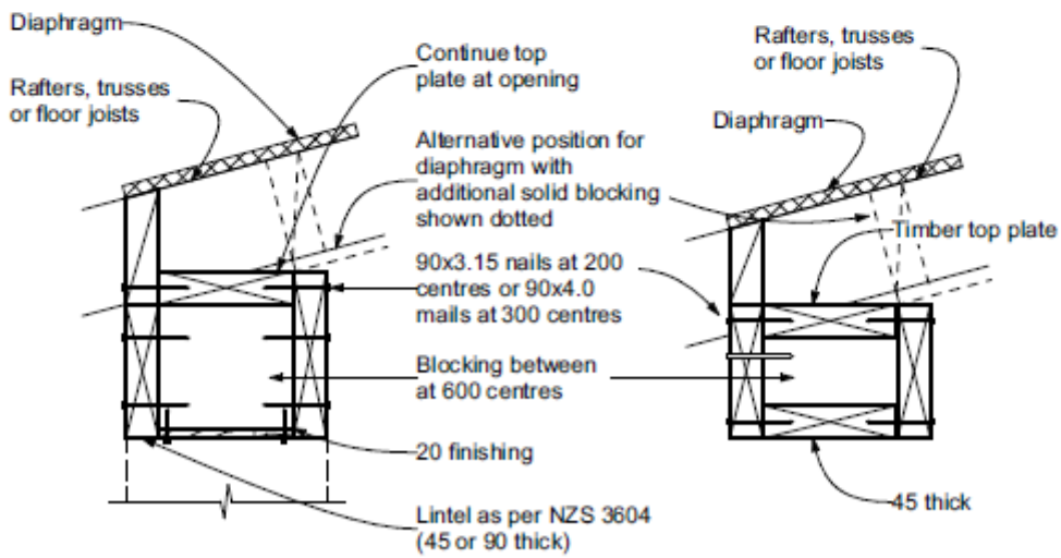
SECTION AT LINTEL
