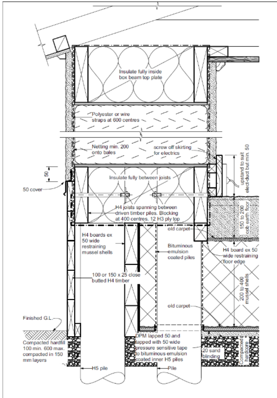
Figure E.10 – External wall on driven timber piles to SED
