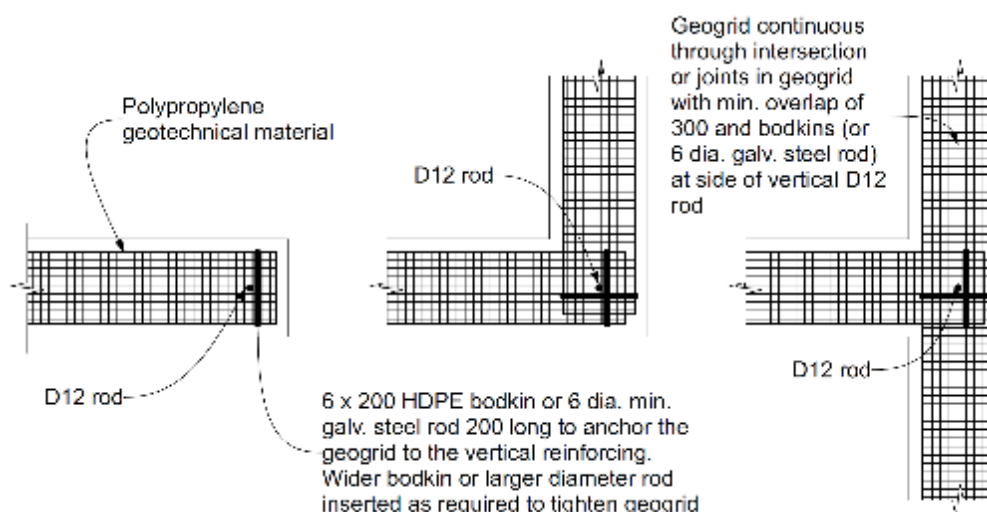
Figure 6.5 – Horizontal reinforcement for earth walls
