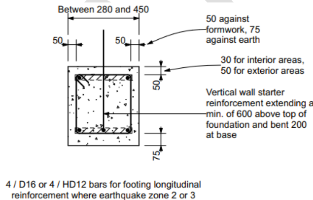
Figure 5.4 – Footing reinforcement in earthquake zone 2 or 3
