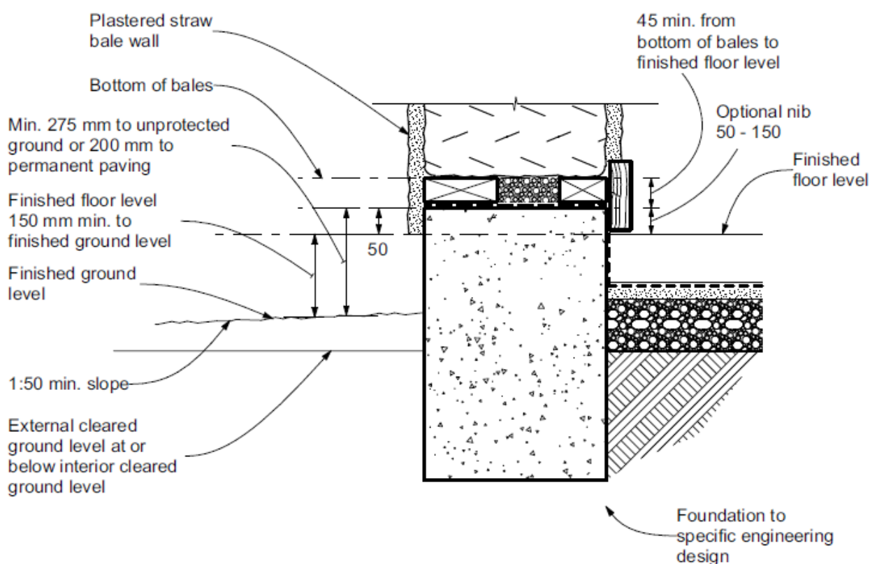
Figure E.1 – Ground clearances
