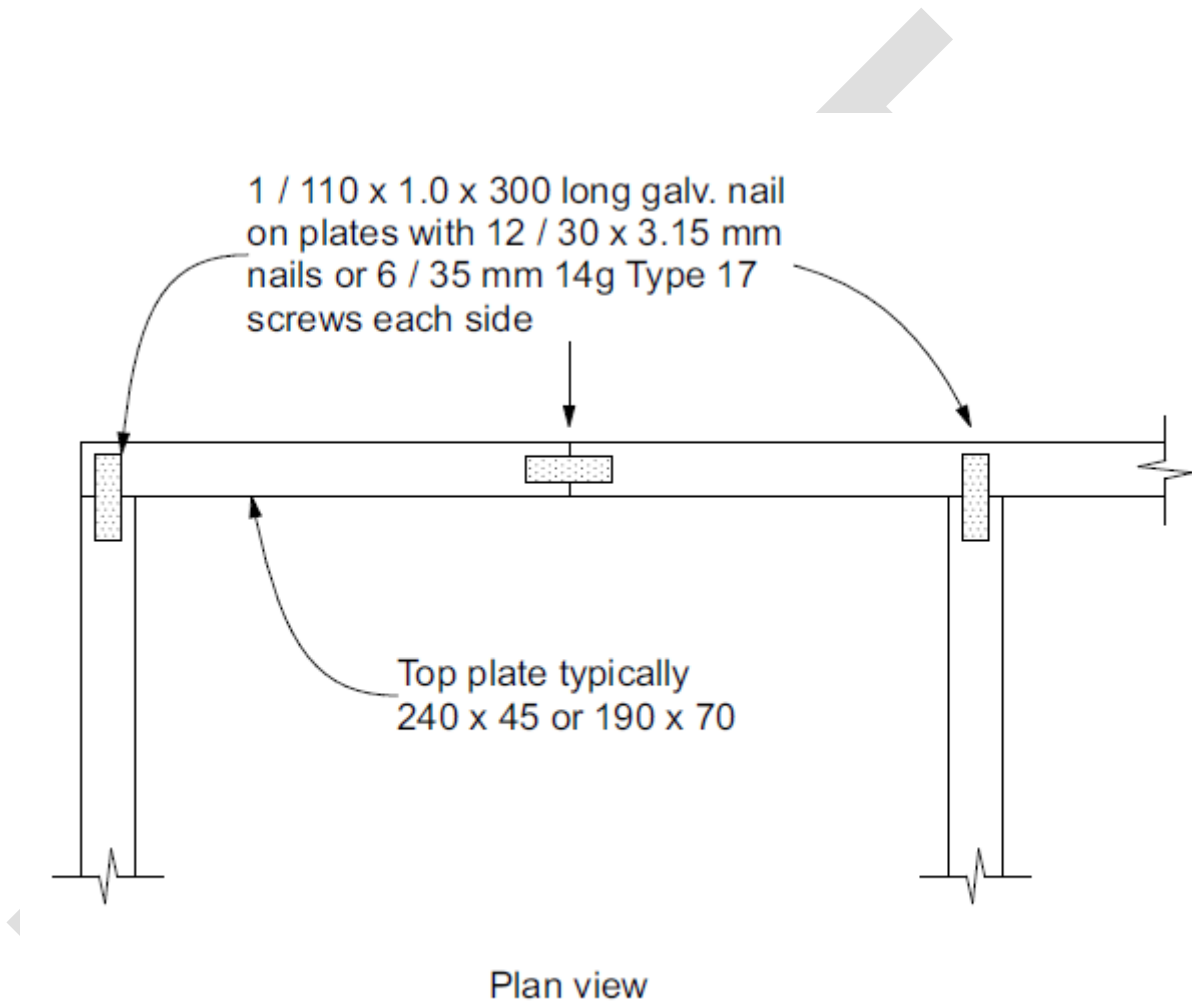
Figure 8.3 – Connection of timber bond beams or top plates with structural diaphragms (plan)
