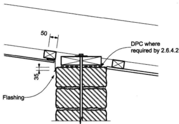
Figure 6.9 – Reverse eaves soffit flashing
