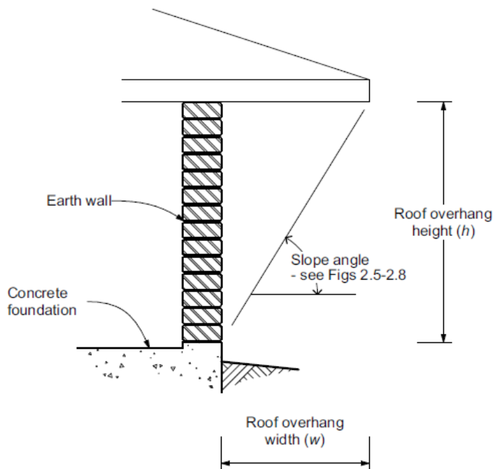
Figure 2.4 - Definition of roof overhang height and roof overhang width
