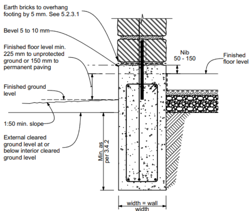
Figure 5.2 – Footing height clearances
