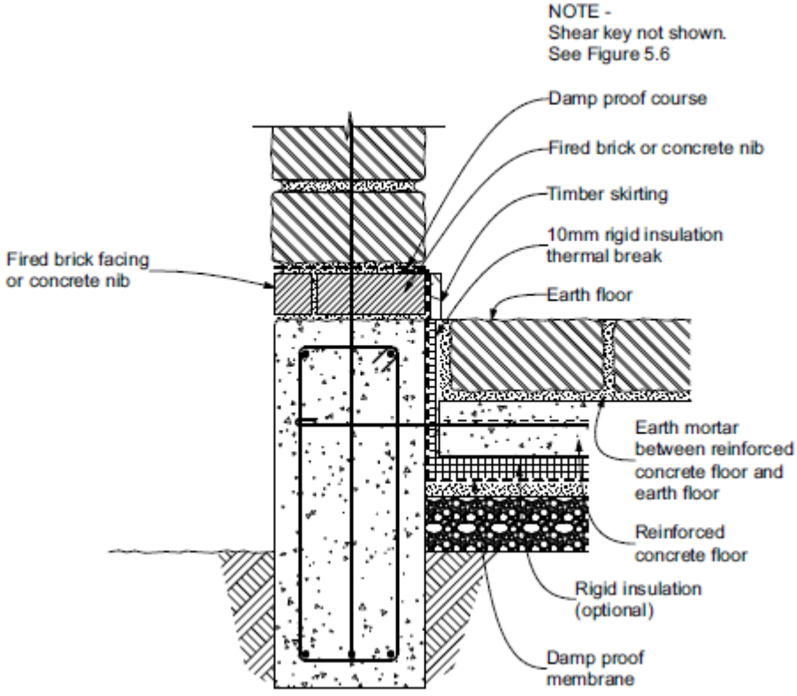
Figure 5.9 – Footing – Insulated earth floor on slab
