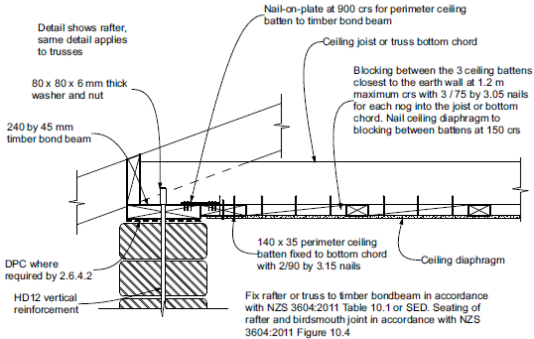
Horizontal ceiling diaphragm - side wall
