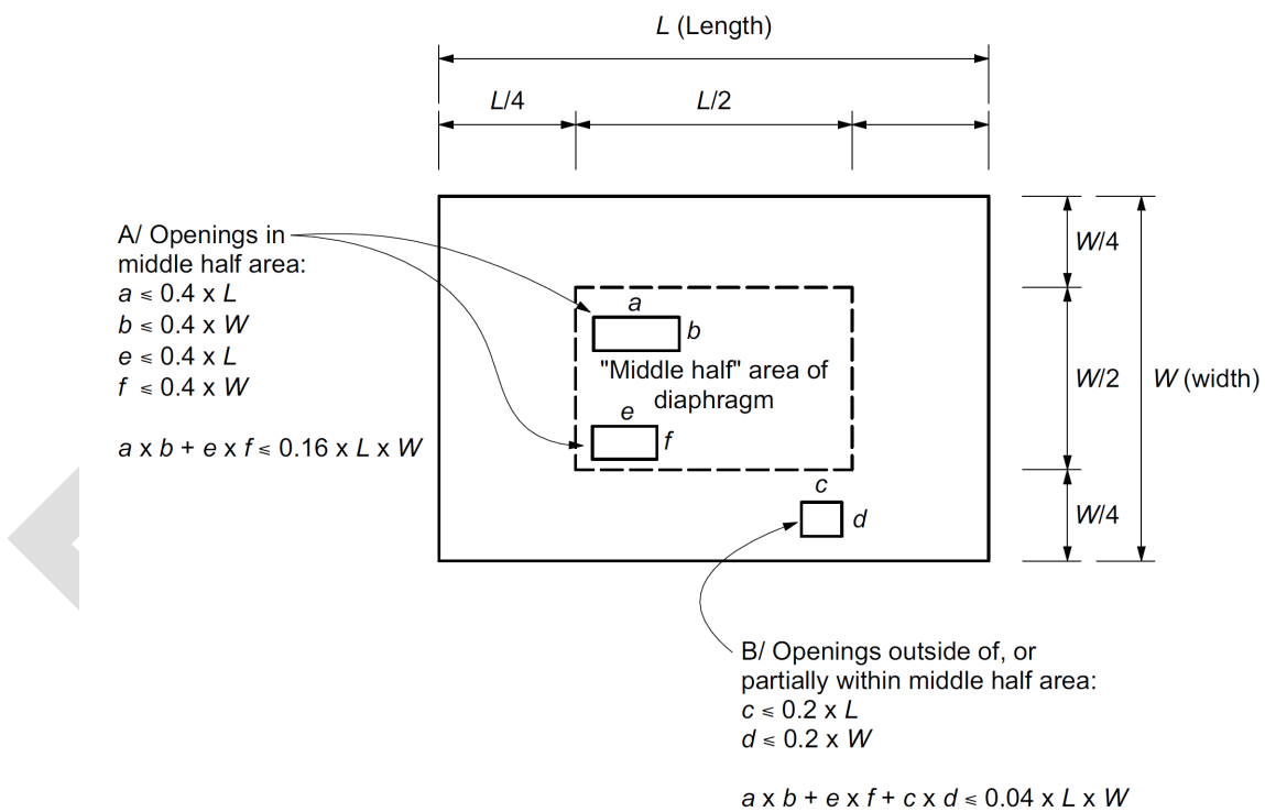
Figure 7.9 Location of opening in diaphragm.
