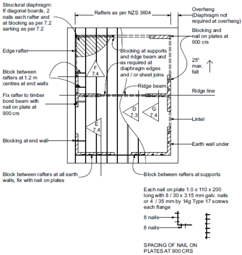
Figure 7.2 – Sloping roof diaphragm
