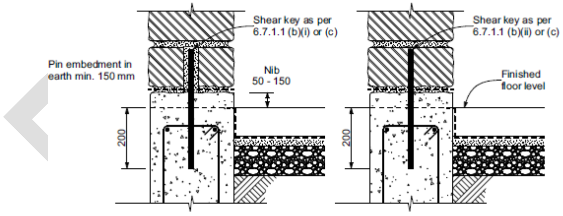
Figure 5.5 – Footings –general details including shear key options
