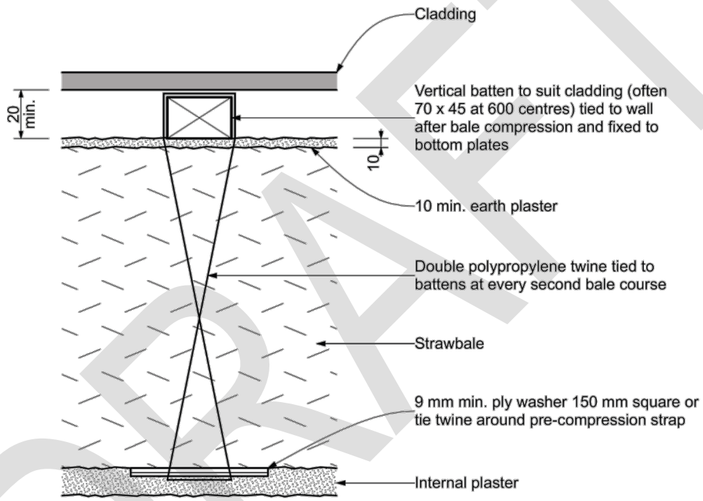
Figure E.8 – Batten tied to straw bale
