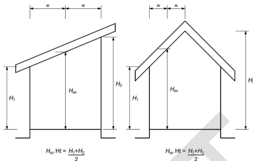
Figure 6.2 – Determining average wall height
