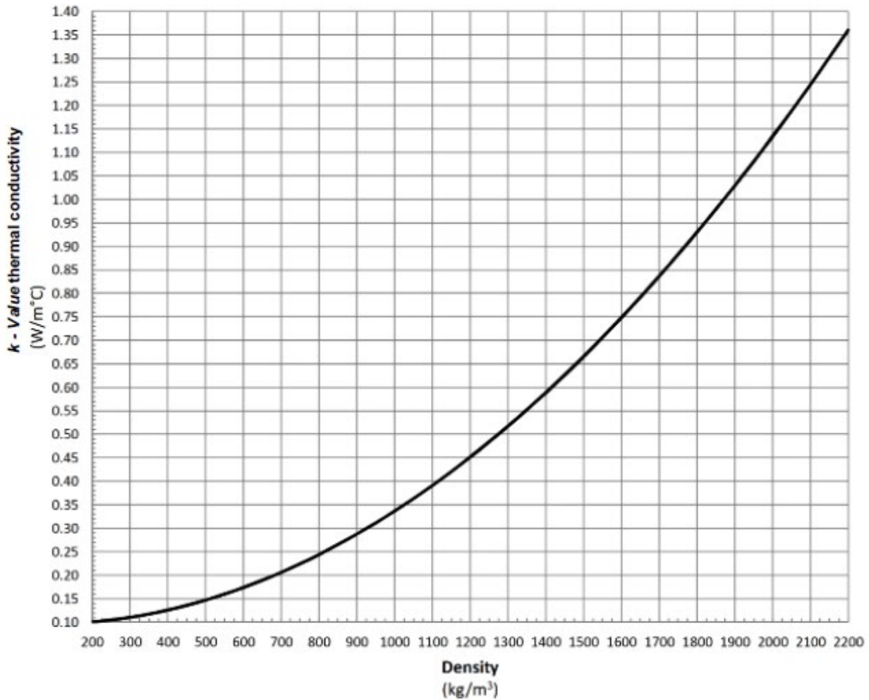
Figure 2.10 – Thermal conductivity values for earth walls
