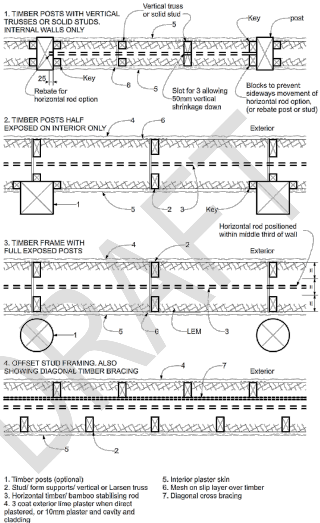
Figure D.1 – Some diagrammatic only framing options for LEM
