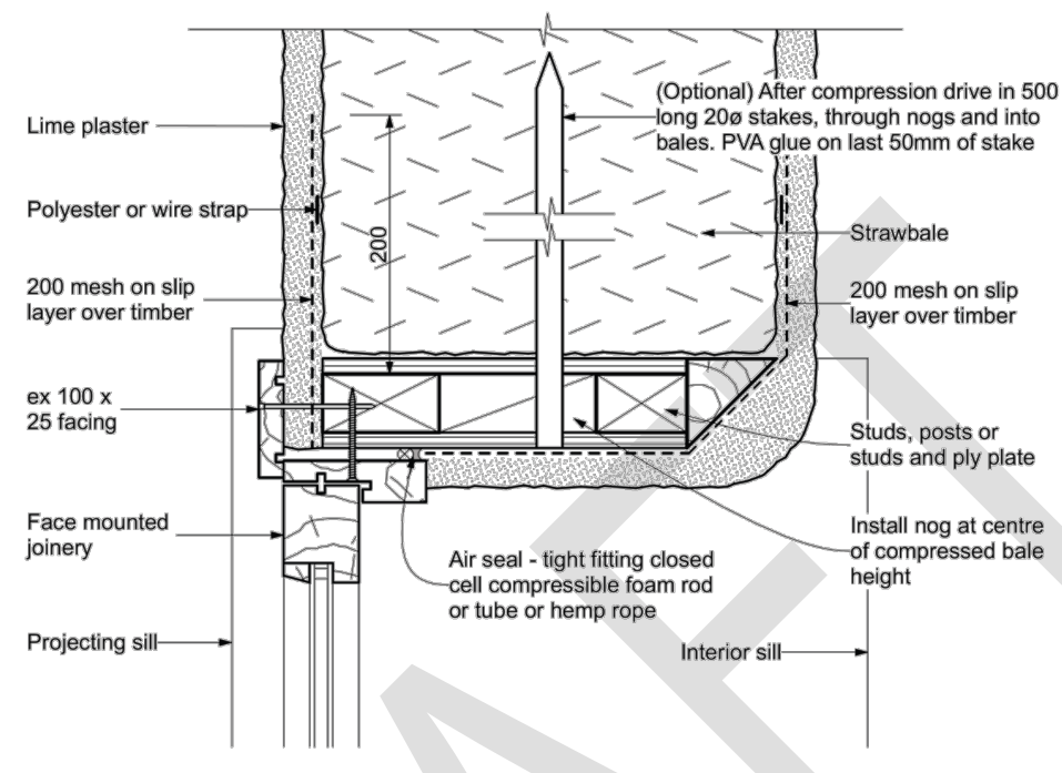
Figure E.3 – Jamb for sheltered walls direct plastered
