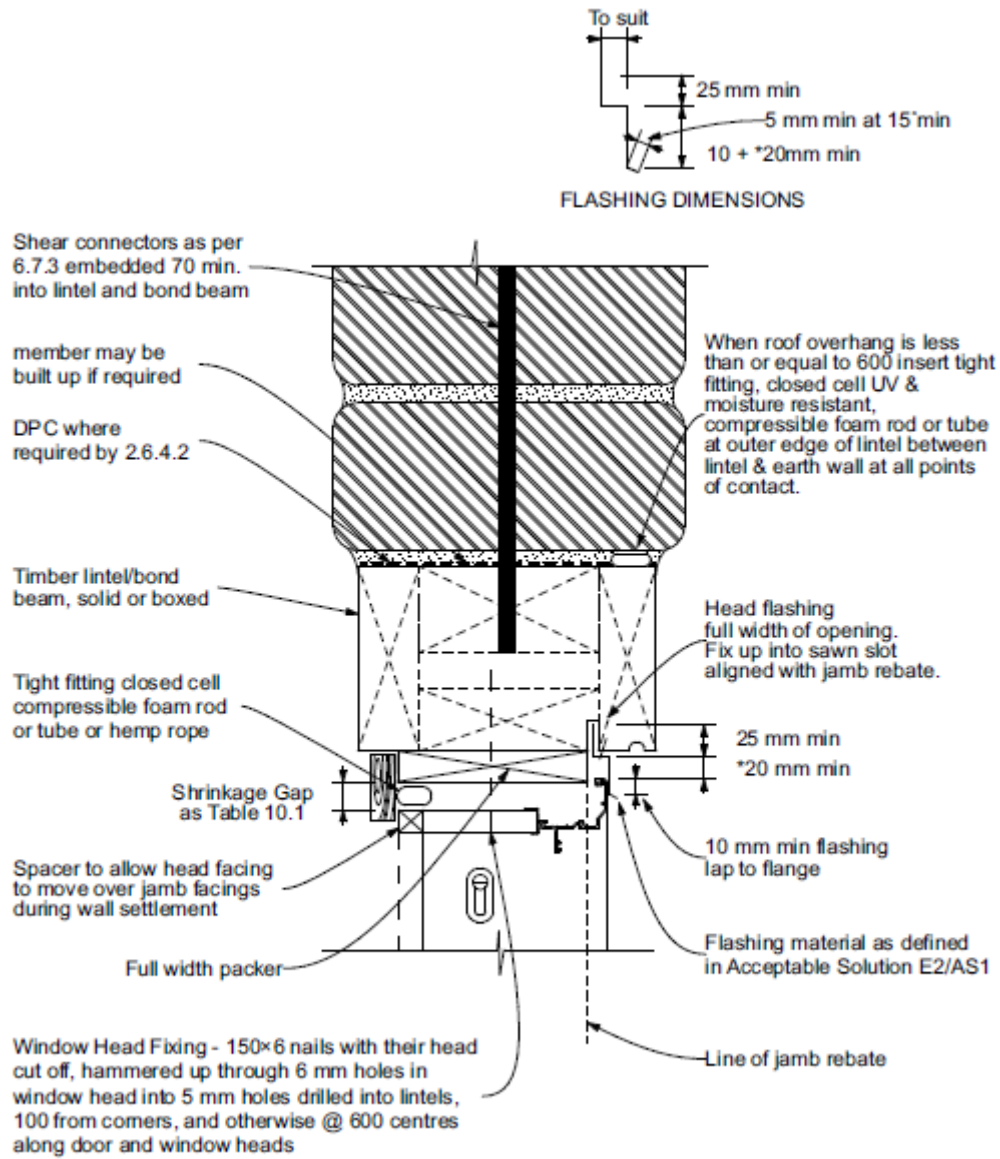
Figure 10.4 – Window head – Aluminium joinery with timber lintel
