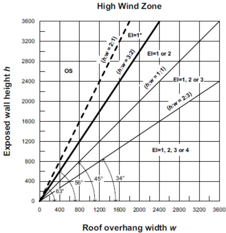
Figure 2.7 - Minimum roof overhang width for high wind zone
