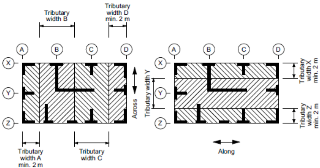
Figure B.1 – Example building 1
