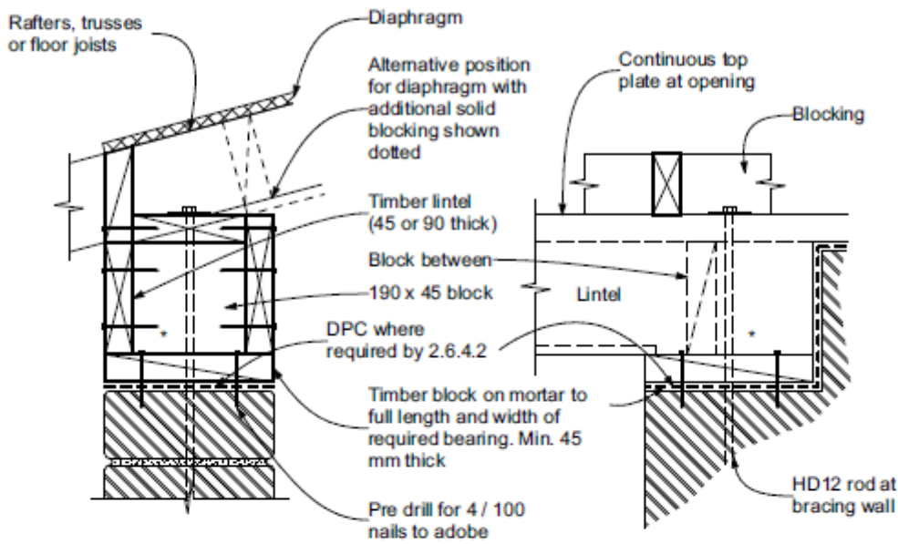
SECTION AT SUPPORT
