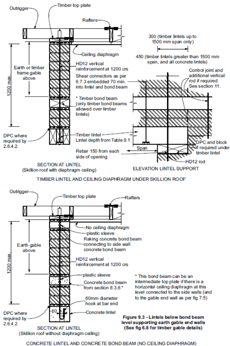
Figure 9.3 – Lintels below bond beam level supporting earth gable end walls (See fig 6.8 for timber gable details)
