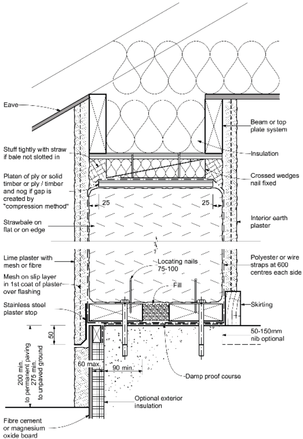
Figure E.7 Straw-bale wall with direct plaster
