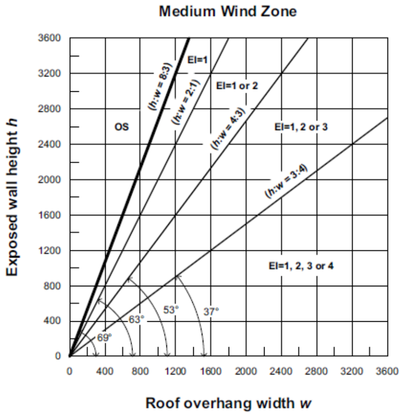
Figure 2.6 - Minimum roof overhang width for medium wind zone
