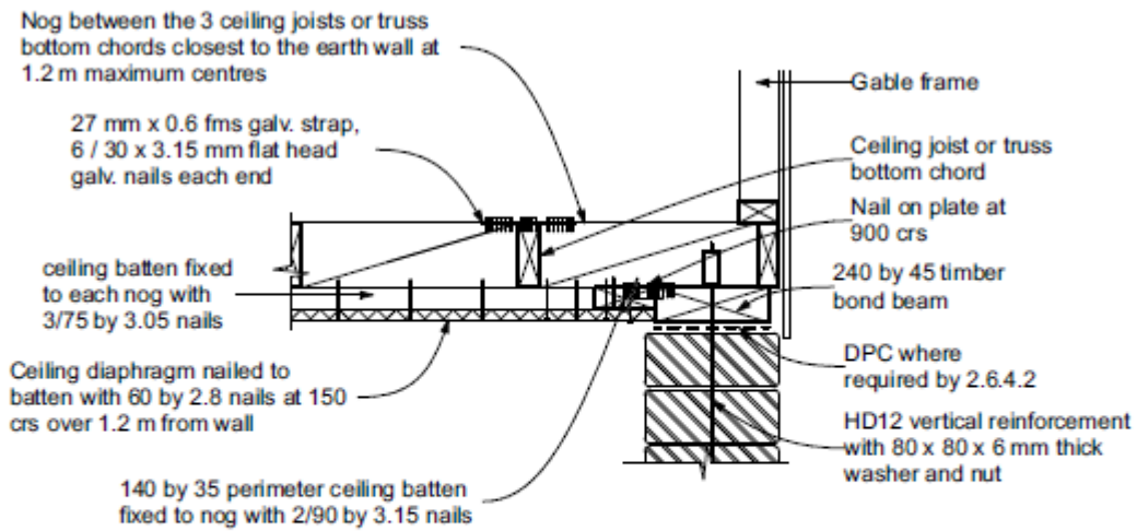
Horizontal ceiling diaphragm - timber gable wall
