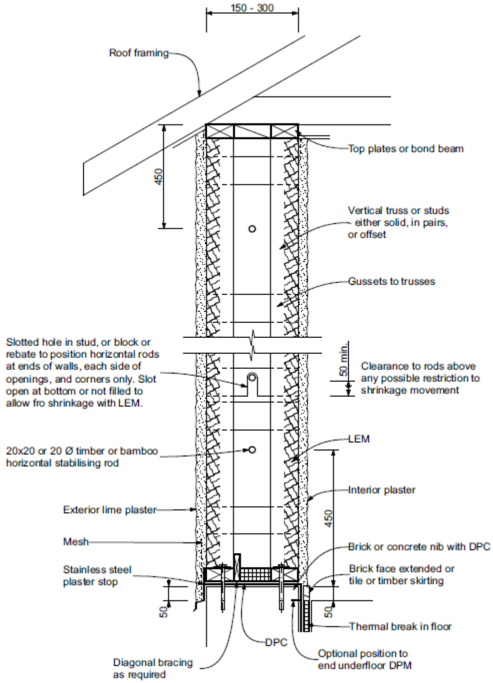
Figure D.4 – LEM wall section
