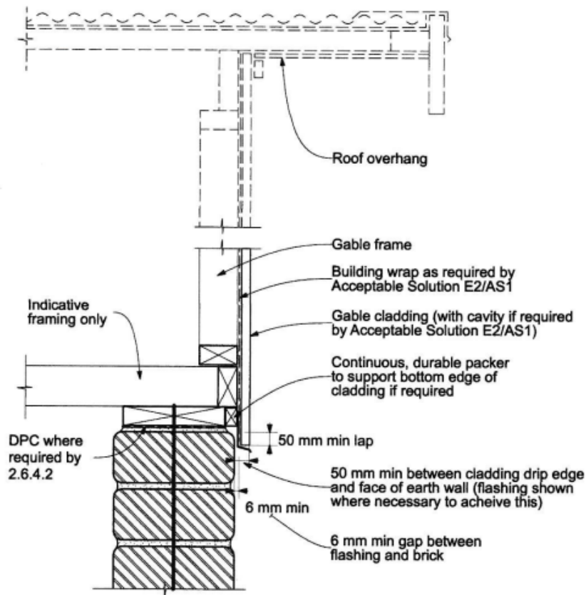
Figure 6.8 – Timber-framed gable to end wall
