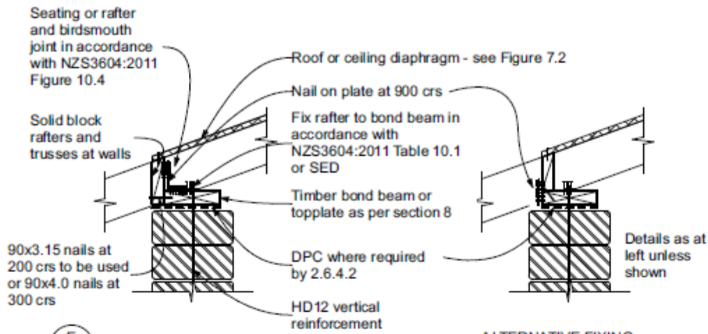
TIMBER BOND BEAM
