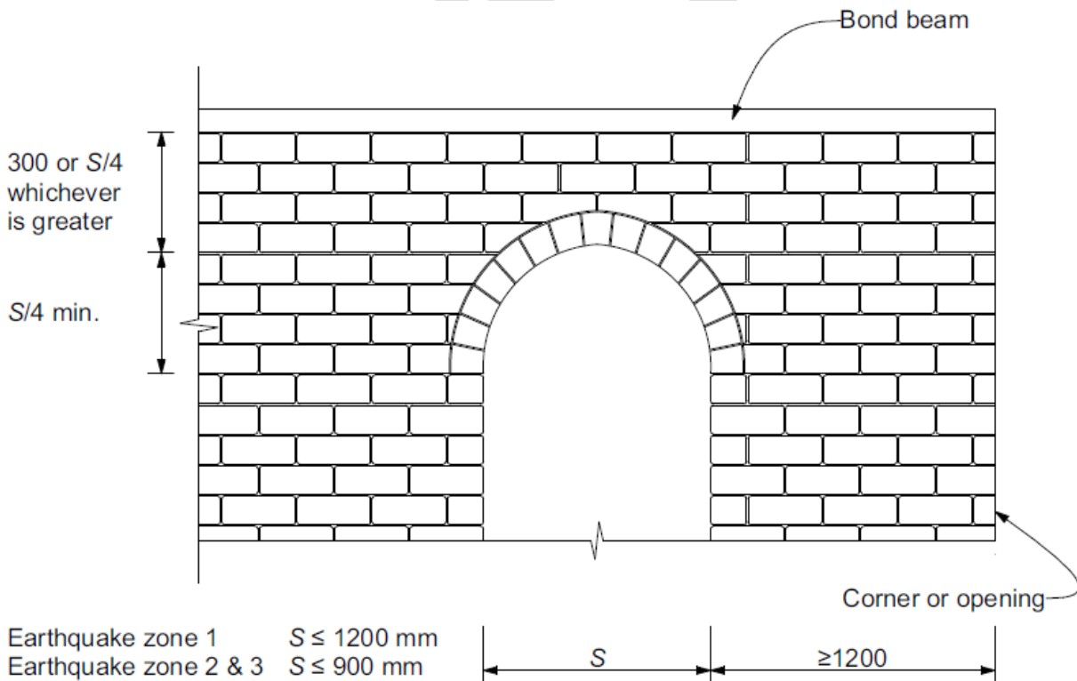
Figure 10.17 - Arch at door, window or opening
