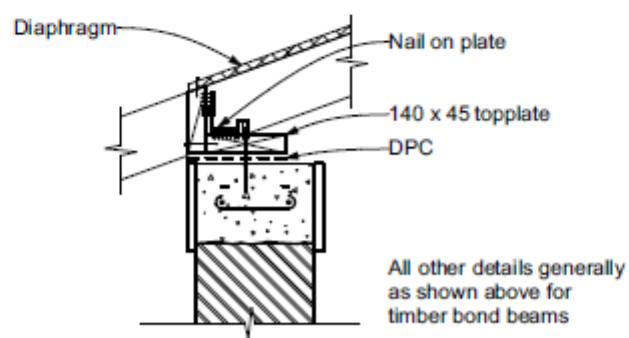
CONCRETE BOND BEAM WITH STRUCTURAL DIAPHRAGM
