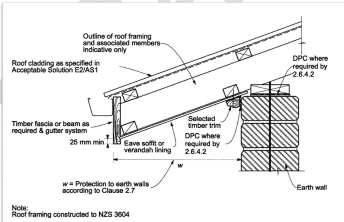
Figure 6.6 – Soffit-to-wall junction
