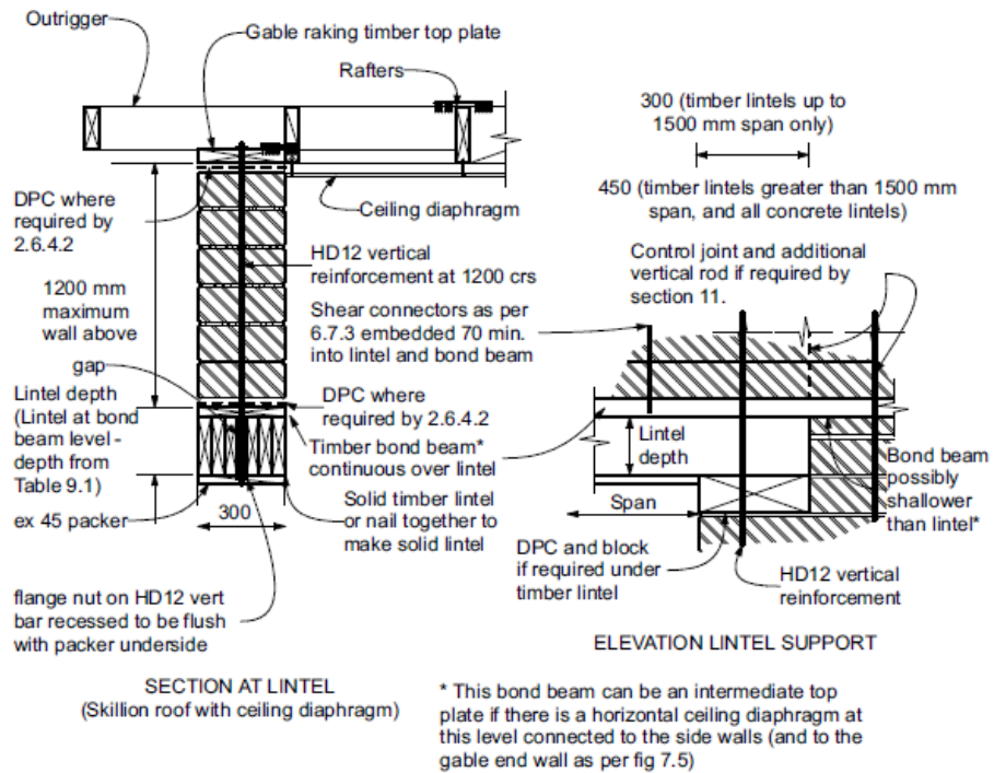
Figure 9.4 – Timber lintel at bond beam level supporting earth gable end walls (see fig 6.8 for timber gable details)
