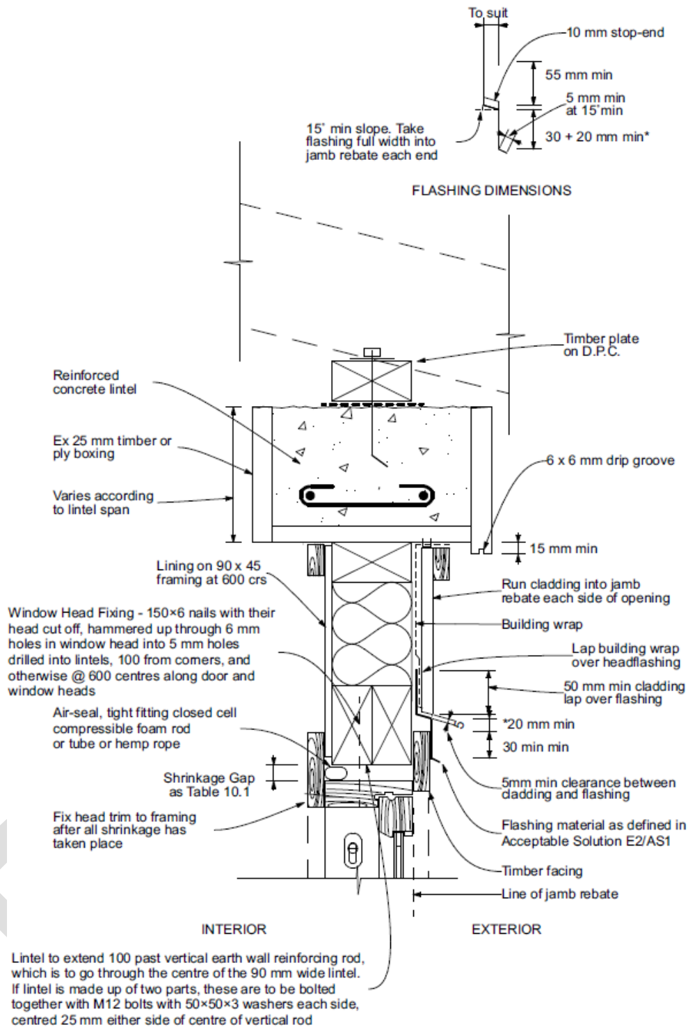
Figure 10.1 – Window head – Timber joinery with timber-framed wall insert
