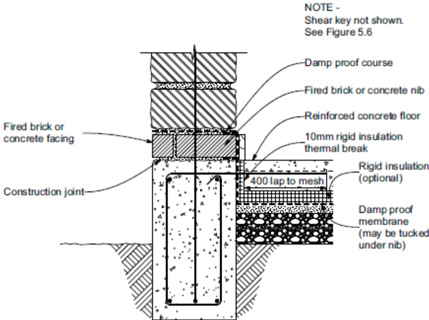
Figure 5.6 – Footing – Insulated concrete floor
