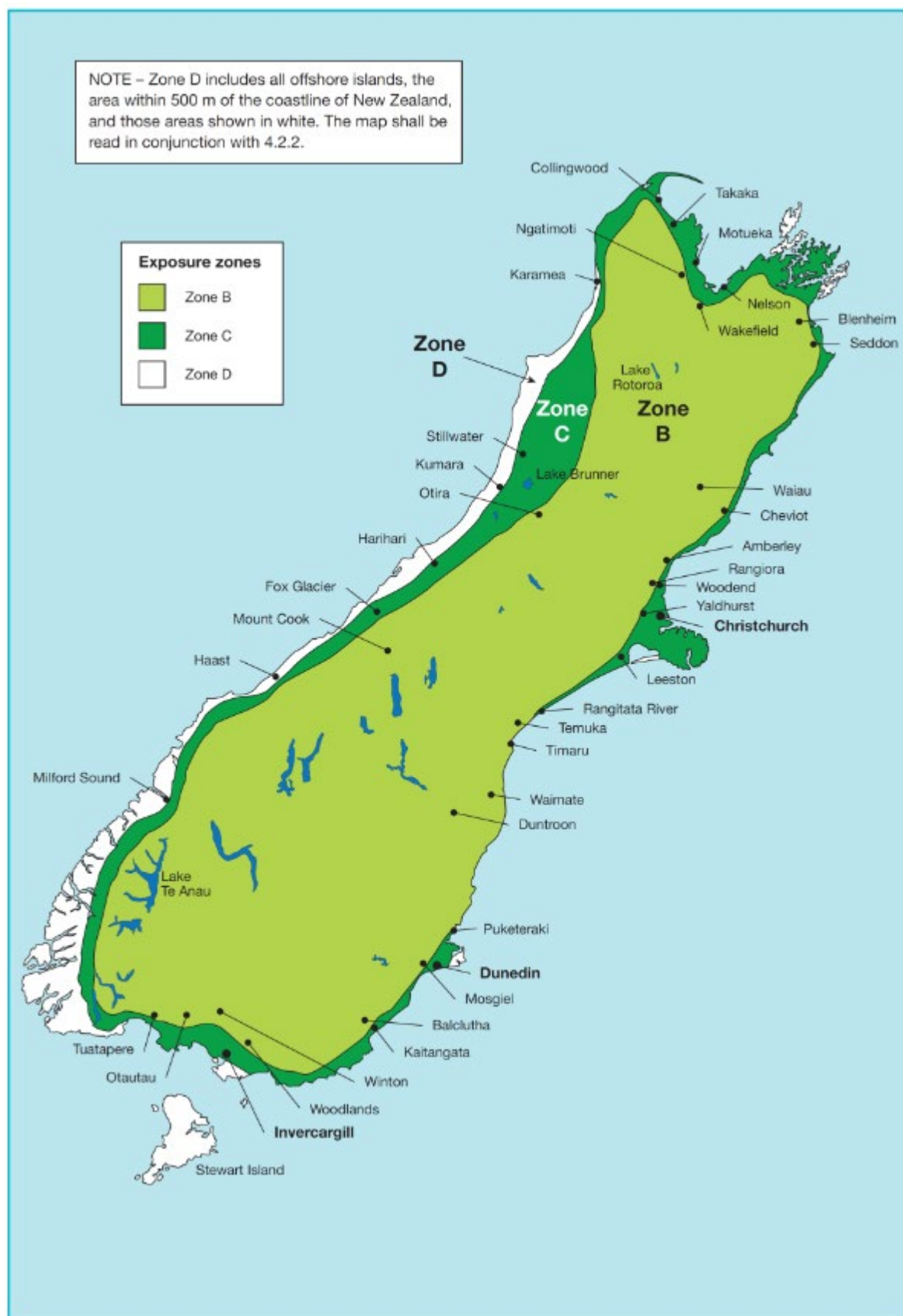
Figure 2.3 – Exposure zone map (South Island)
