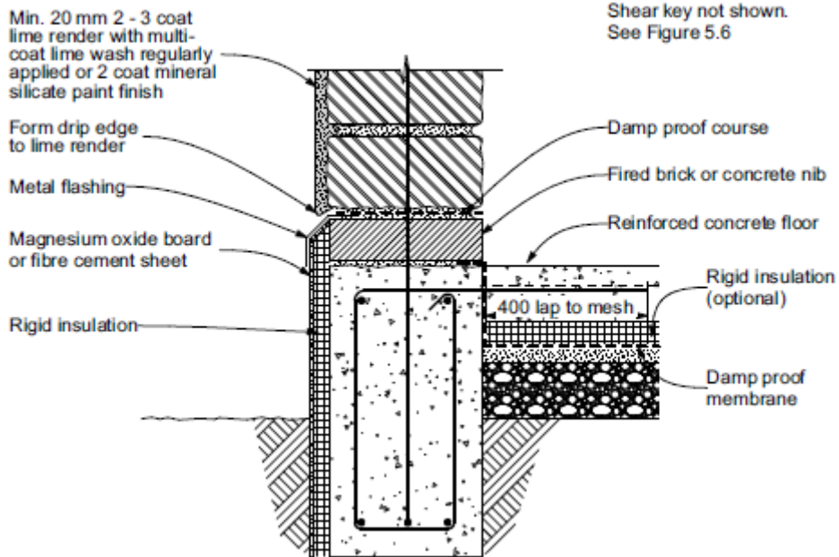
Figure 5.12 - Footing - Insulated footing and slab for lime render over solid earth wall
