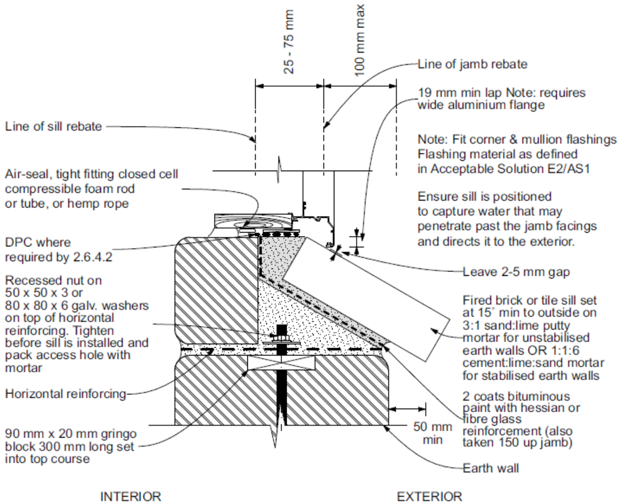
Figure 10.8 – Window sill – Aluminium joinery with brick or tile sill
