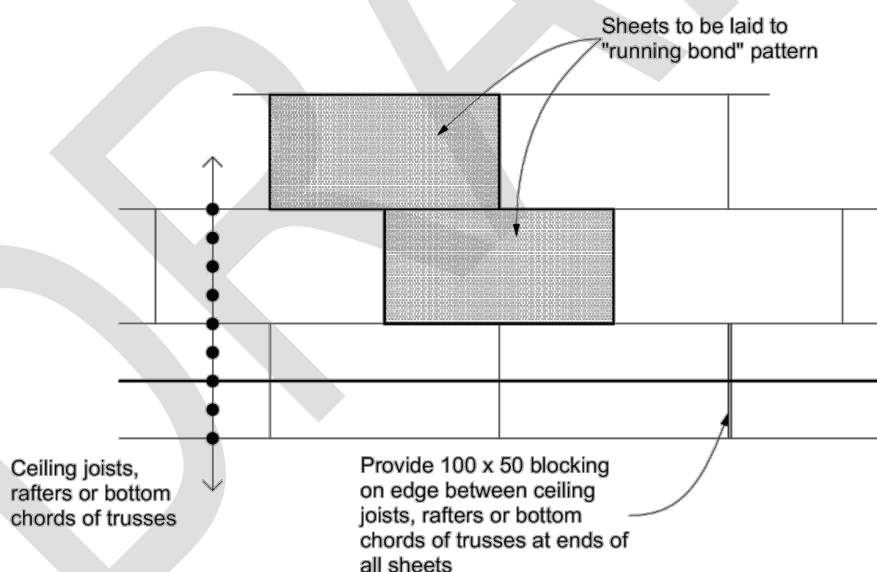
Figure 7.1 – Diaphragm construction (see 7.1.2)
