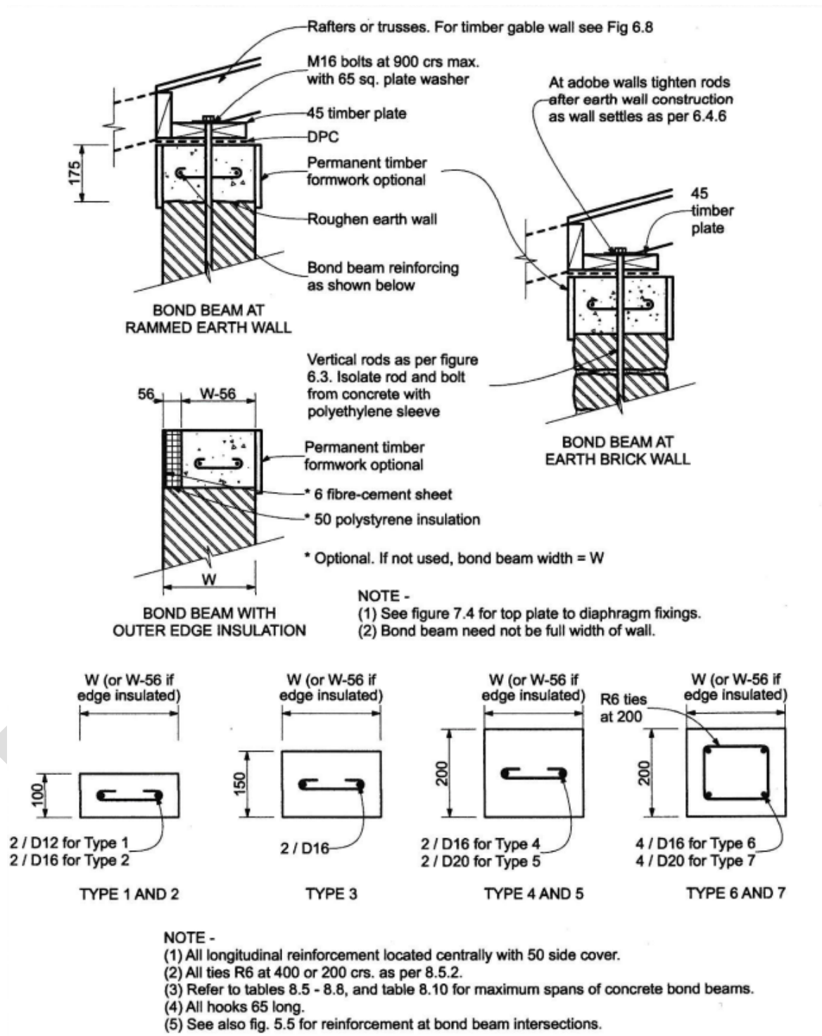
Figure 8.5 – Concrete bond beams
