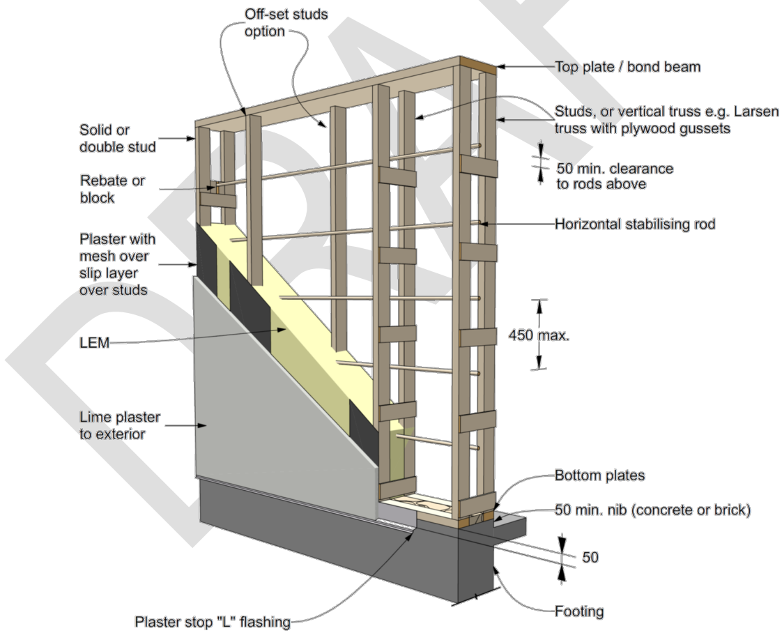
Figure D.2 – Drained vented cavity to LEM
