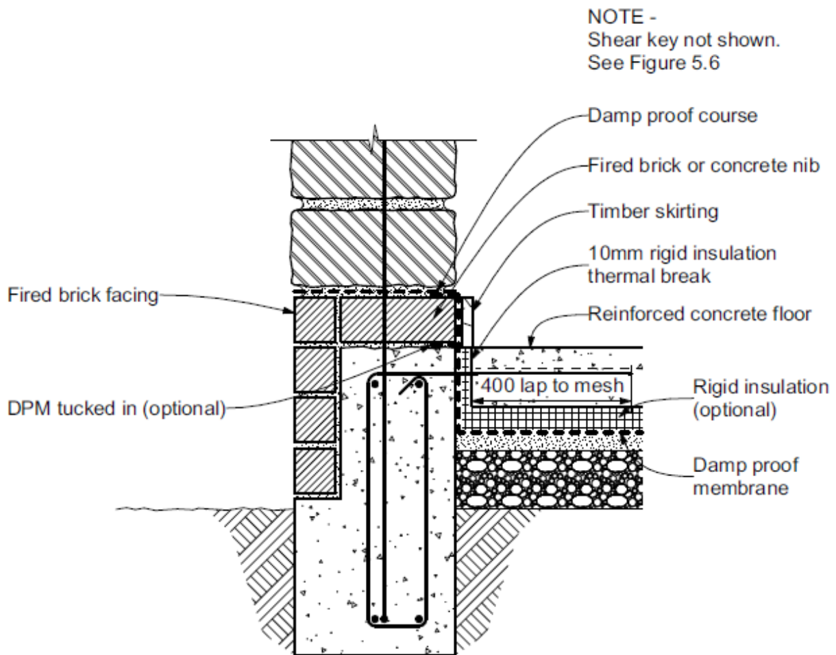
Figure 5.8 – Footing – Insulated slab with brick facing
