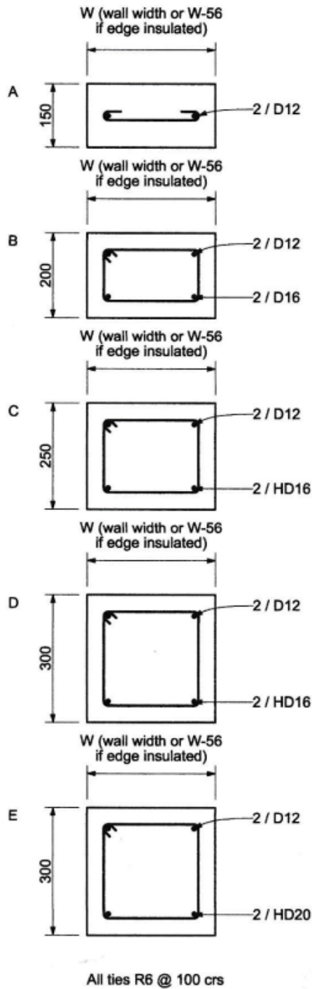
Figure 9.7 – Concrete lintel sizes and reinforcement
