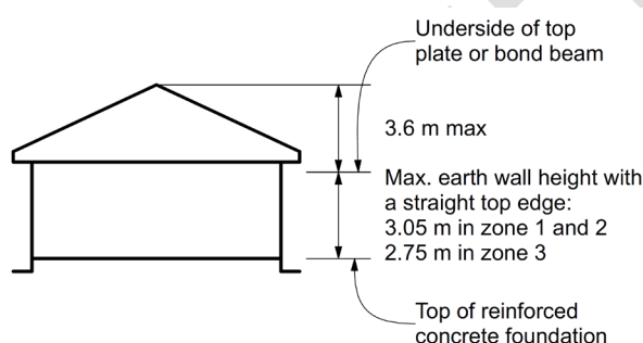
B Height limitations roofs or timber-framed gable ends
