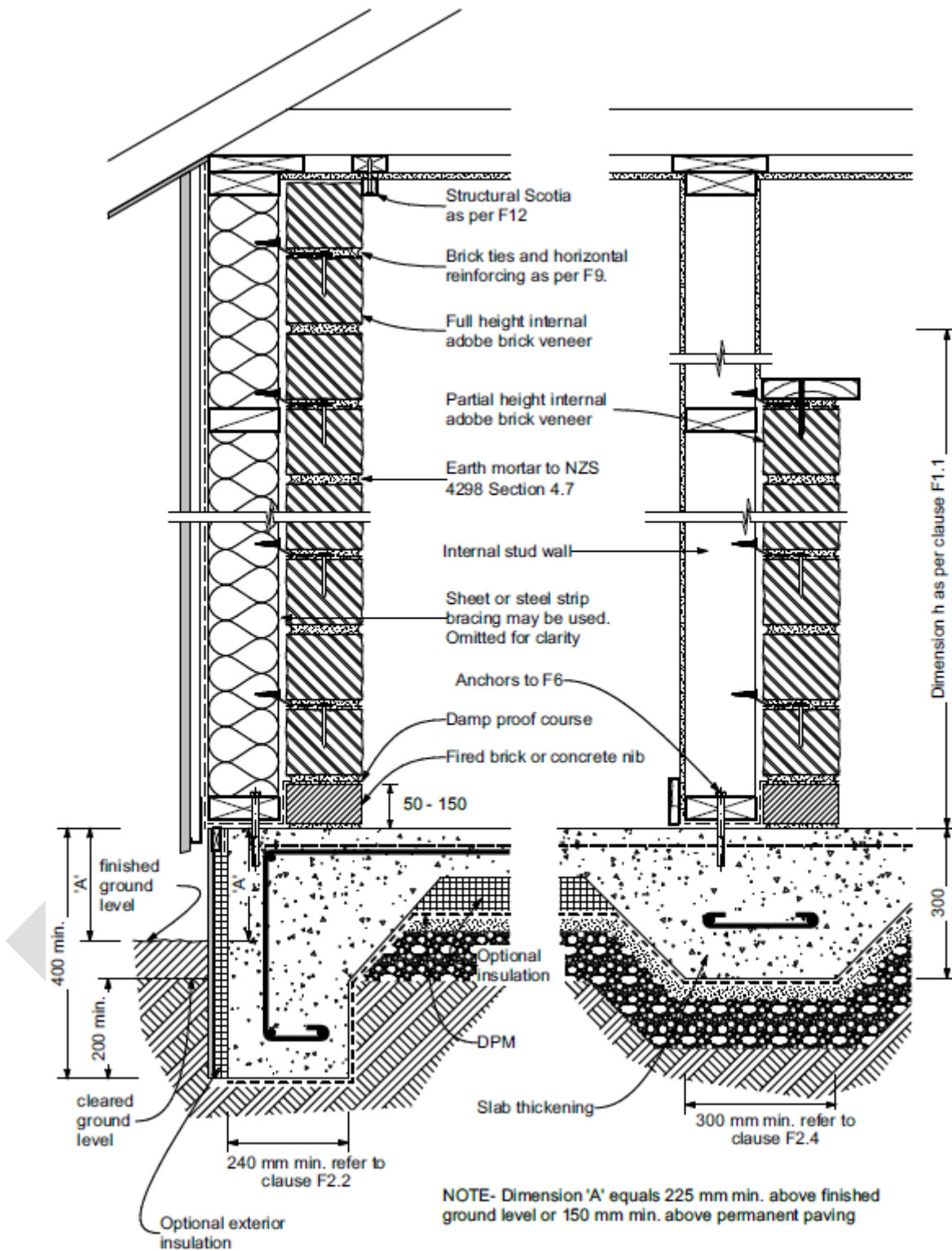
Figure F.1 – Internal veneer details
