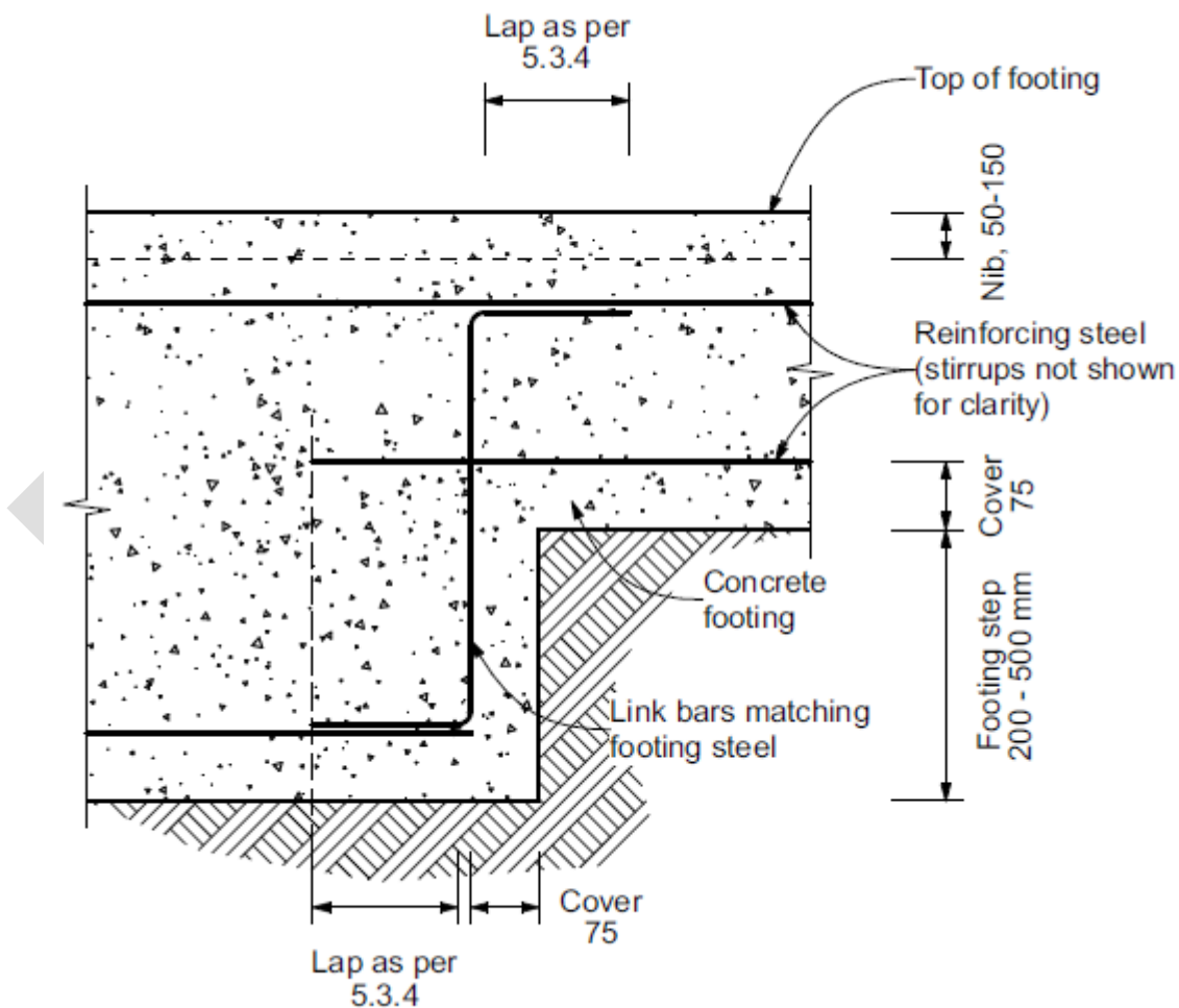
Figure 5.1 – Foundation details at footing step
