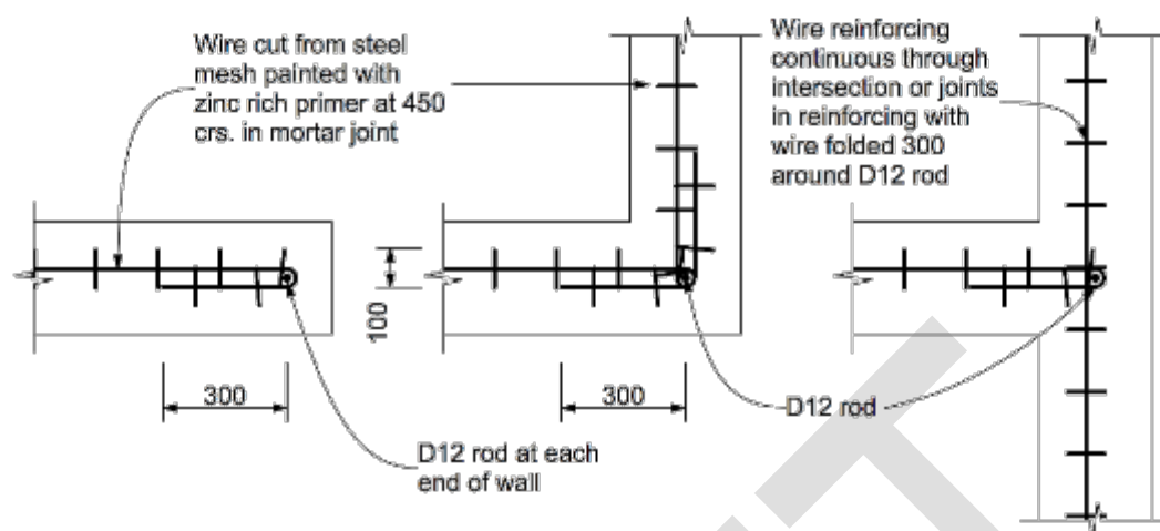
Figure 6.4 – Horizontal reinforcement cut from steel mesh
