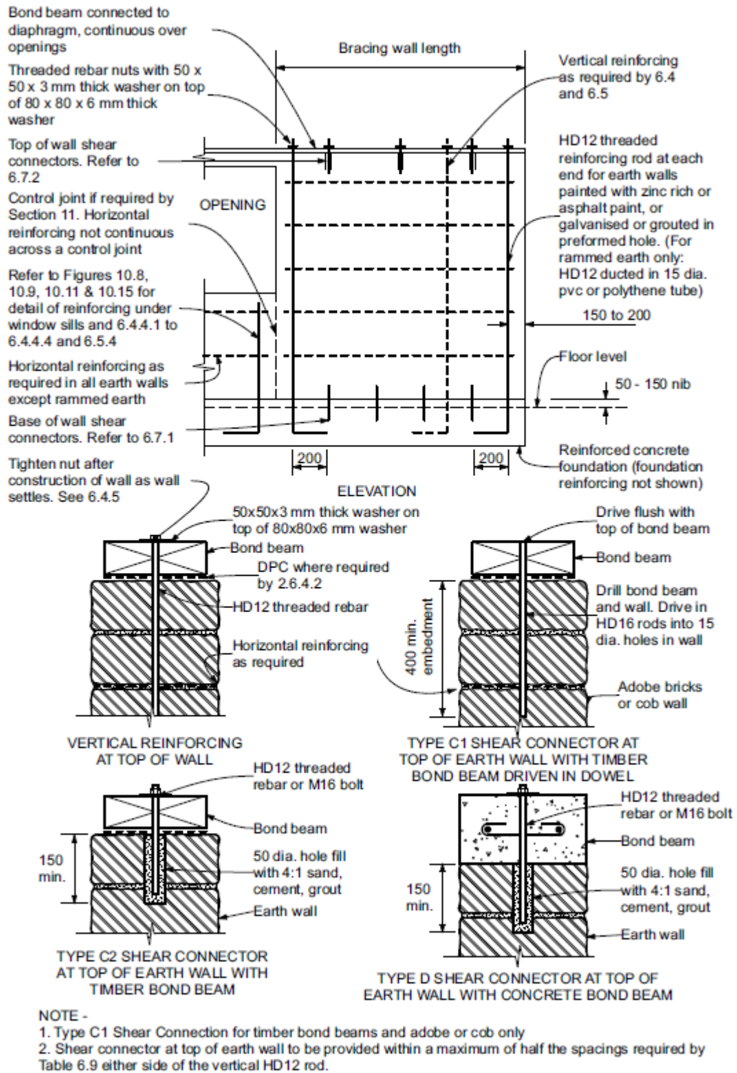
Figure 6.3 – Reinforcing and shear connectors for reinforced earth walls
