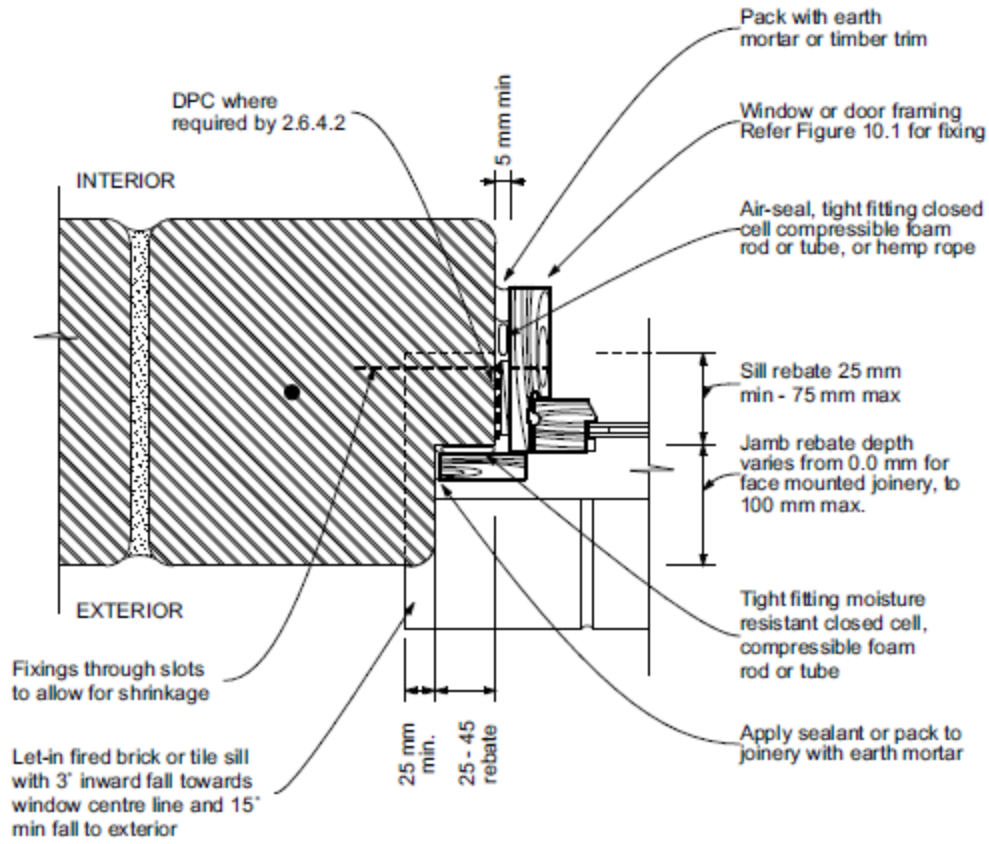
Figure 10.5 – Window jamb – Timber joinery
