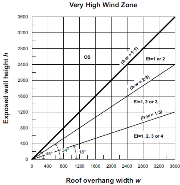
Figure 2.8 - Minimum roof overhang width for very high wind zone
