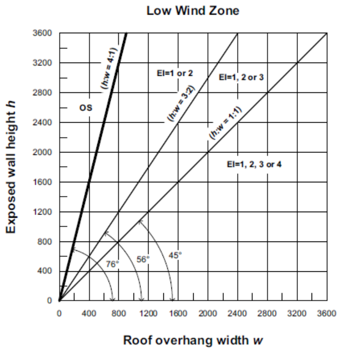
Figure 2.5 - Minimum roof overhang width for low wind zone 5
