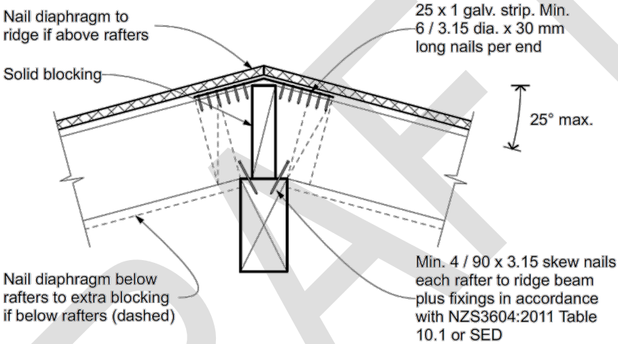
Figure 7.3 – Sloping roof diaphragm – ridge section
