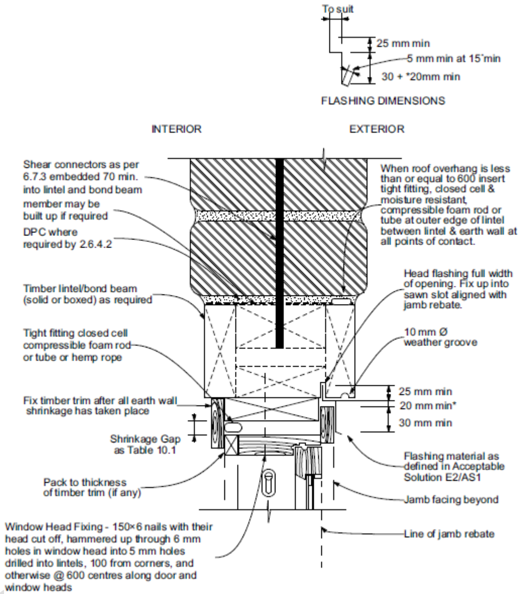
Figure 10.3 – Window head – Timber joinery with timber lintel
