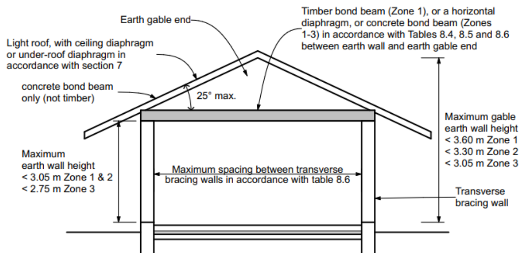
Figure 8.6 – Bond beam for gable end walls above earth walls
