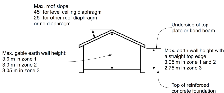
A Height limitation for earth wall gable ends
