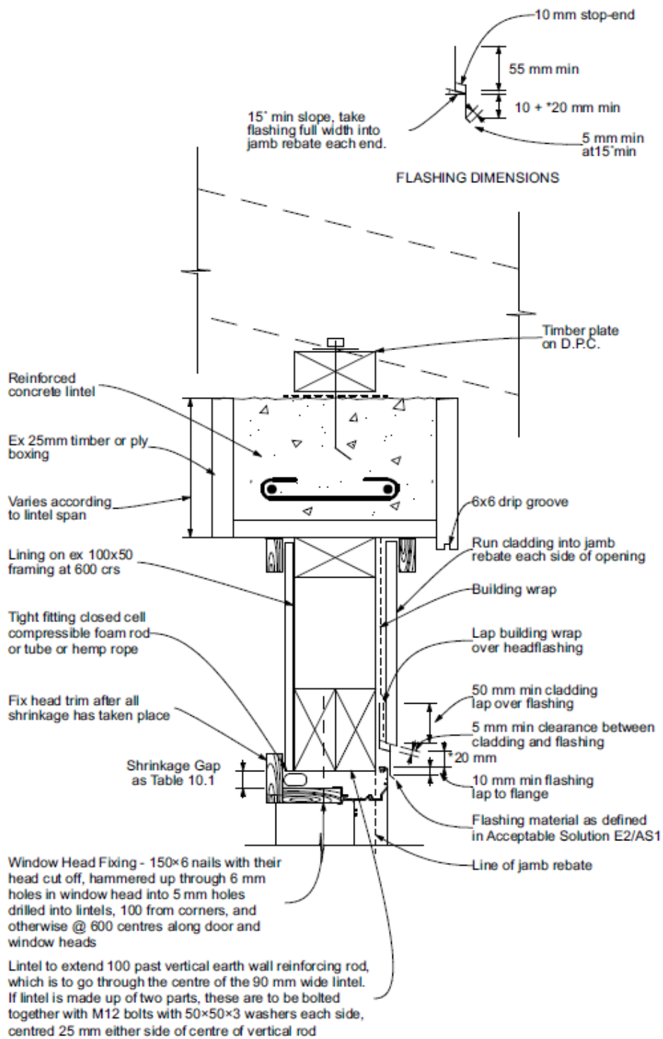
Figure 10.2 – Window head – Aluminium joinery with timber-framed wall insert
