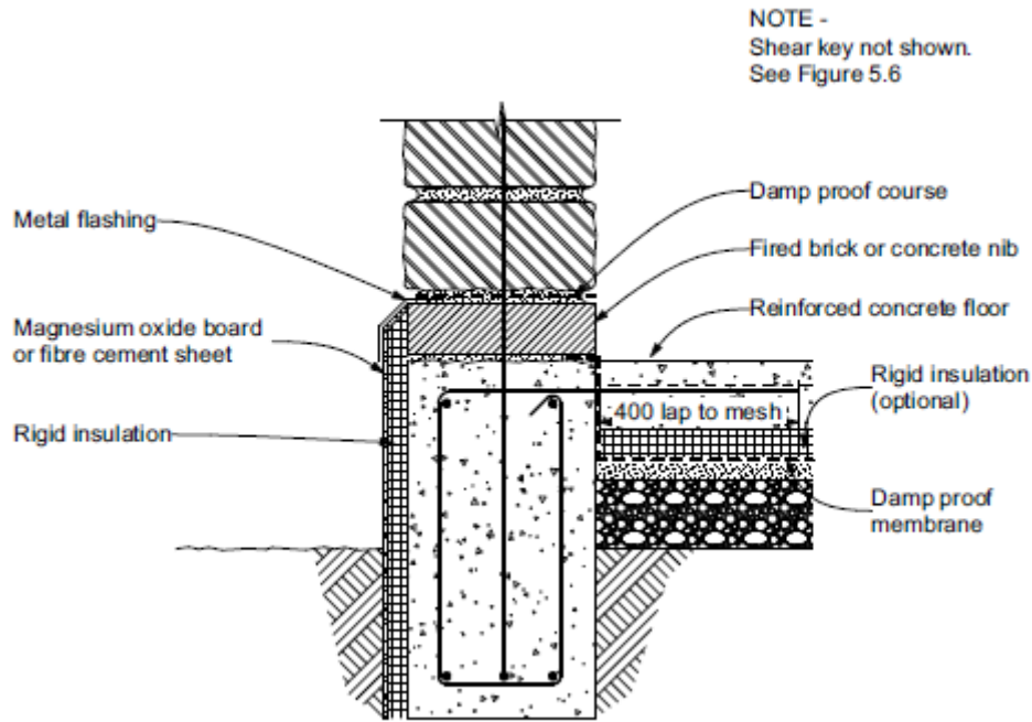
Figure 5.7 – Footing – Insulated slab and footing
