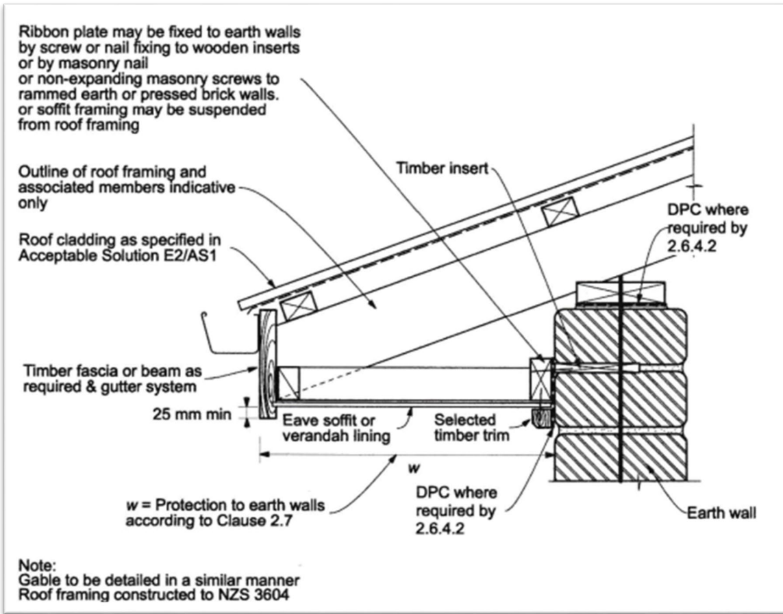
Figure 6.6 – Soffit-to-wall junction
