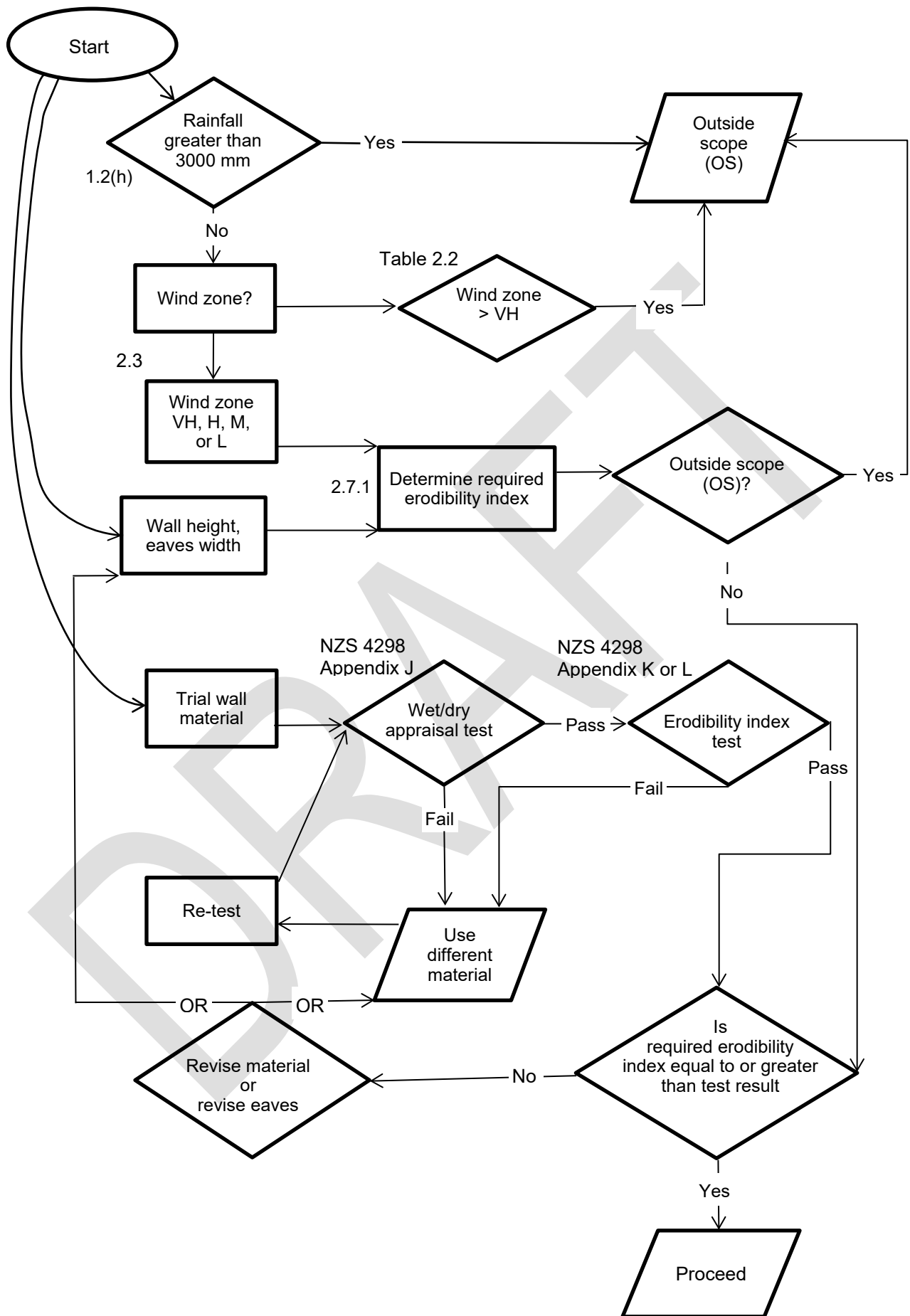
Figure 2.1 – Durability design
