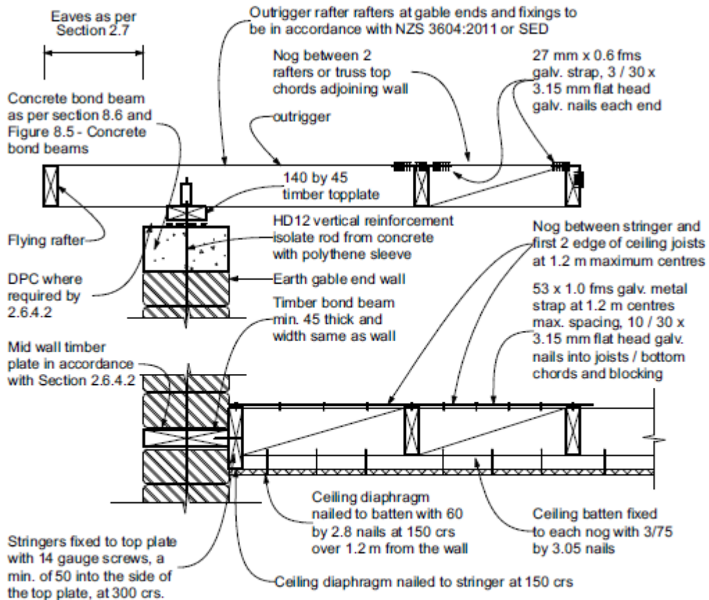
Horizontal ceiling diaphragm - earth gable wall
