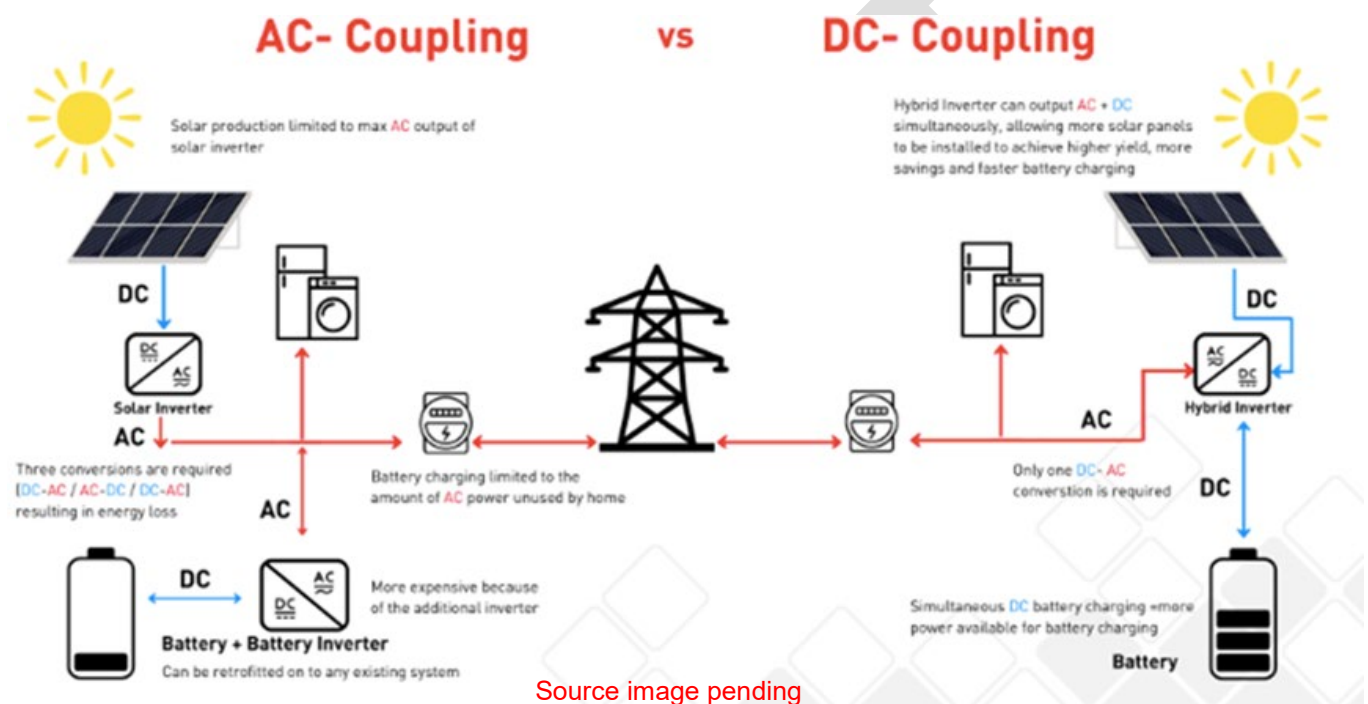
Figure 23 – Typical AC and DC system configurations
